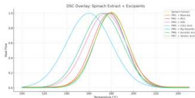
Fig 09 DSC overlay
