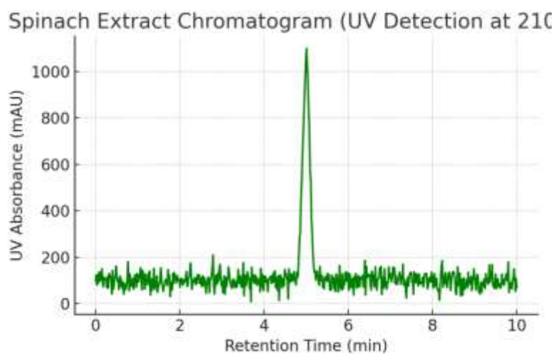
Fig.03 spinach chromatogram
